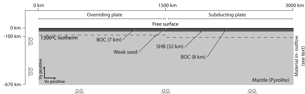
FIGURE 5.9 – Model setup for subduction of a 70 Myr old oceanic plate under a 40 Myr old oceanic plate. The top boundary is free. The bottom and left boundary are free-slip, while the right boundary condition includes material in- and outflow. SHB: Serpentinised Harzburgite, and BOC: Bulk Oceanic Crust.
