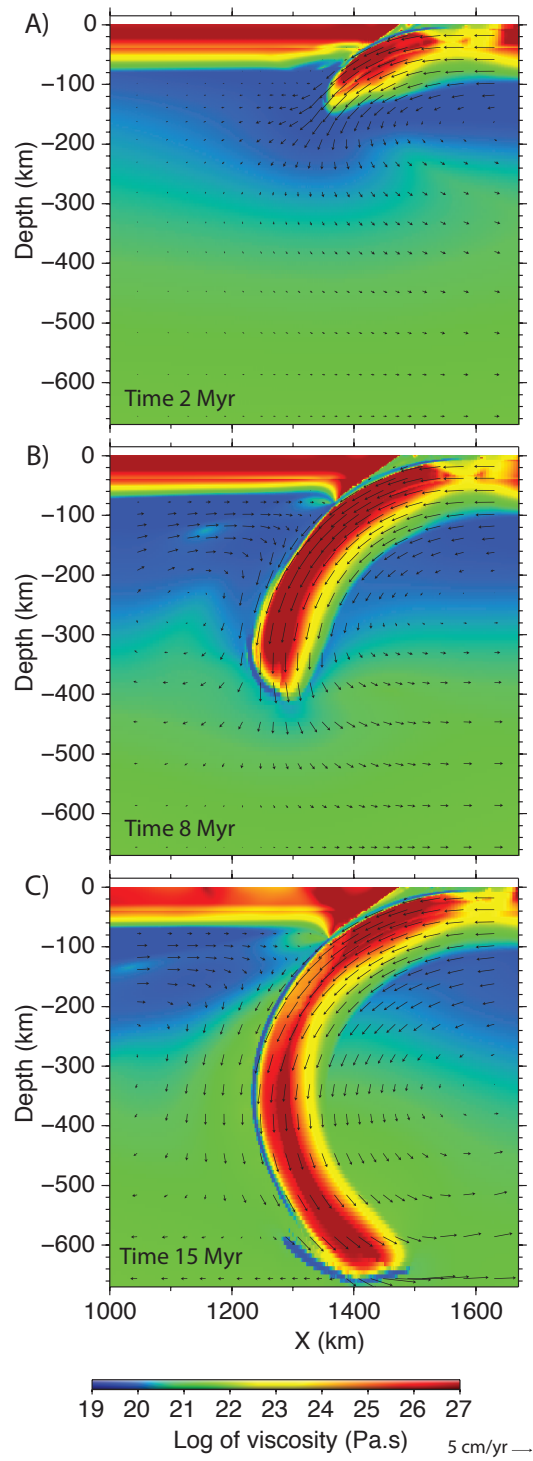
FIGURE 4.13 – Viscosity fields at A) 2 Myr, B), 8 Myr, and C) 15 Myr for thermo-mechanical case 4. The model was calculated with SULEC.
