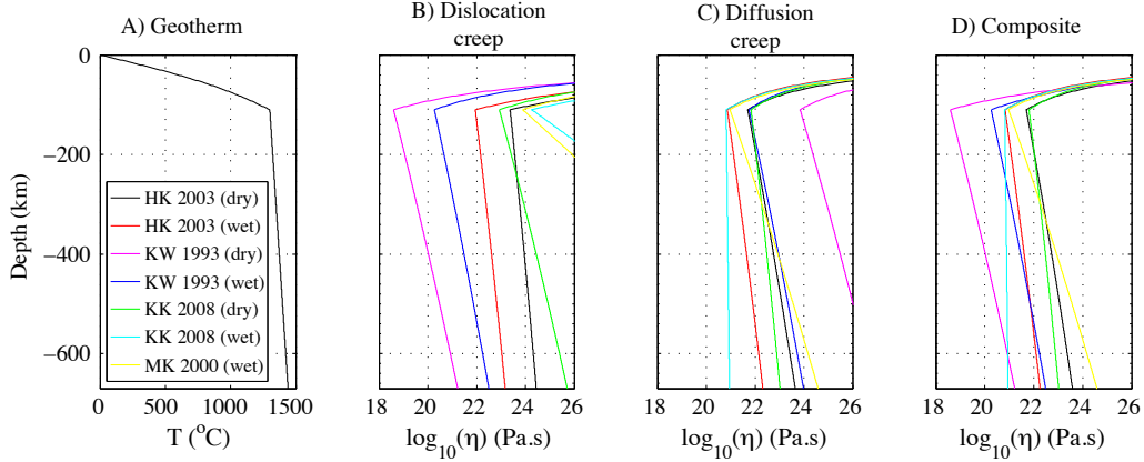
FIGURE 4.1 – A) Oceanic geotherm for a 70 Ma lithosphere. B) Dislocation creep viscosities; C) Diffusion creep viscosities; D) Parallel (composite) diffusion and dislocation creep viscosities (Eq. 4.6). The viscosity profiles in B-D are computed for the 70 Ma geotherm in A). A constant strain rate of 10^{-15} \text{ s}^{-1} and flow law parameters for olivine are used. HK 2003 = Hirth and Kohlstedt (2003) , KW 1993 = Karato and Wu (1993) , MK 2000 = Mei and Kohlstedt (2000a,b) , and KK 2008 = Korenaga and Karato (2008) .
