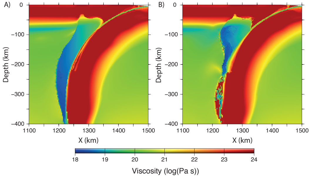
FIGURE 5.16 – Viscosity fields in the mantle wedge for subduction models calculated using the imposed free water migration scheme II with v_{f,y} = 5 \text{ cm yr}^{-1} . A) Only the effects of bound water are taken into account in the viscosity calculations (using a maximum cut-off for C_{\text{OH}} of 0.4 wt % in Eq. 5.4). This is the same model as Fig. 5.10B. B) The effects of both bound and free water are taken into account in the viscosity calculations (using a maximum cut-off for C_{\text{OH}} of 1 wt % in Eq. 5.4).
