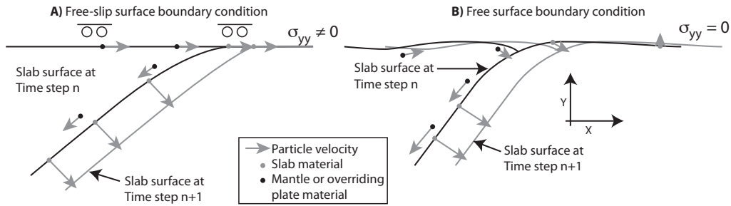
FIGURE 3.12 – Simple schematics of the effects of A) free-slip and B) free surface boundary conditions on the particles located at the trench (see text).
