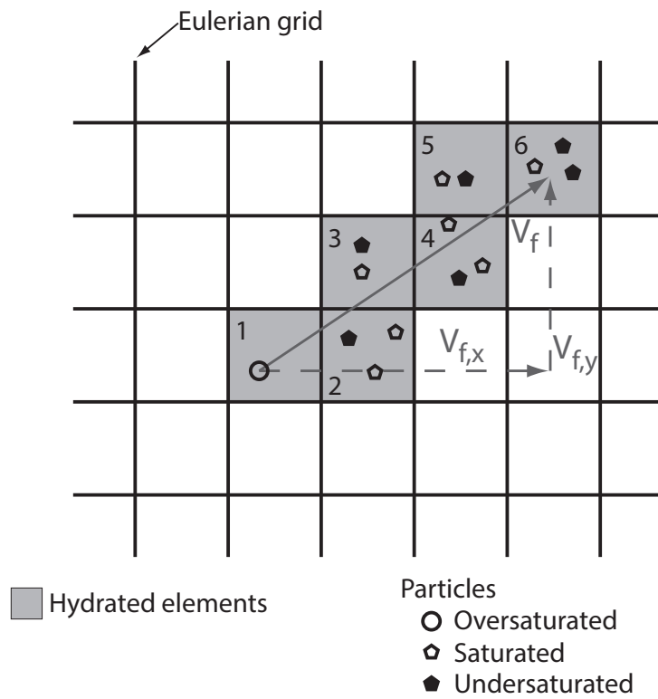
FIGURE 5.3 – Schematic migration of free water and it's distribution along a prescribed path for our velocity controlled water migration schemes II and III (see text for further explanation). V_f is water velocity.
