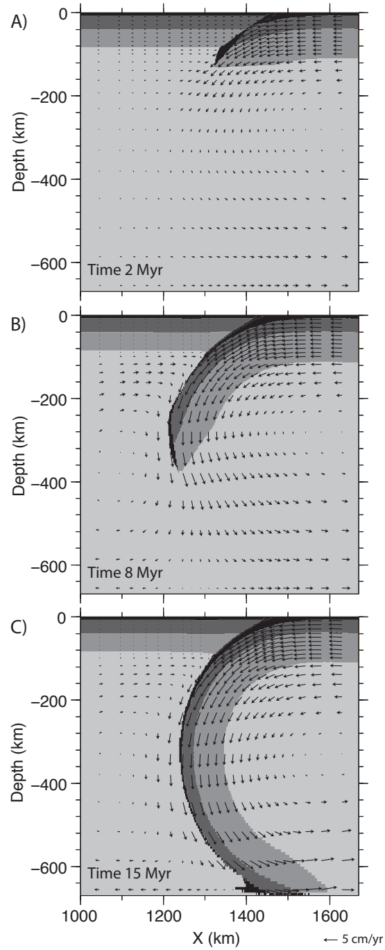
FIGURE 4.4 – Subduction evolution for linear viscous case 1, calculated using SULEC. The materials are shown for a 670 km wide region (from the total 3000 km model width), focused on the trench.
