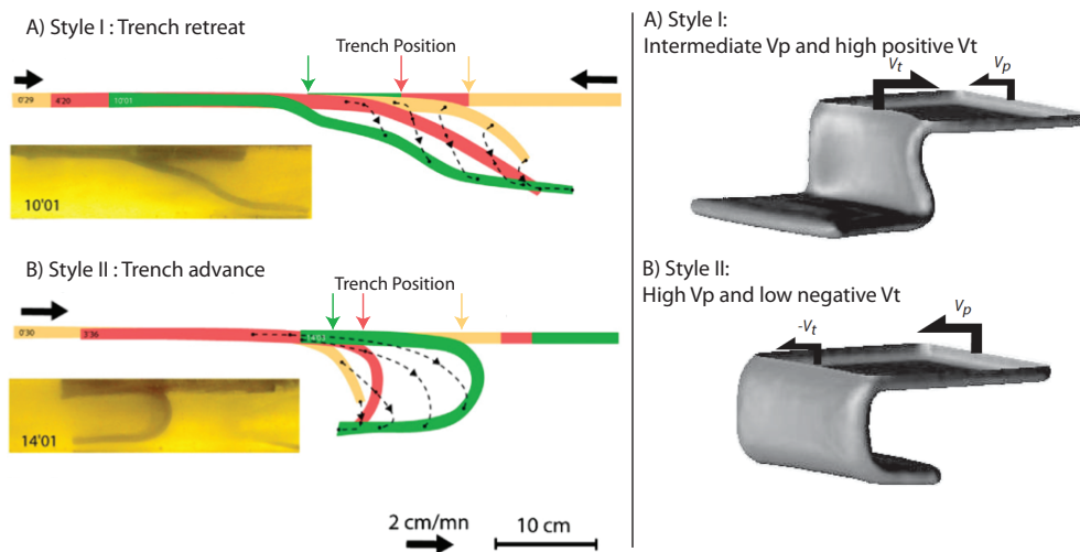
FIGURE 1.4 – Two main styles of deformation of the subducting lithosphere during free subduction obtained using analogue models (left column from Heuret et al. (2007)) and numerical models (right column from Di Giuseppe et al. (2009)). V_t is the trench velocity or the velocity of the overriding plate and V_p is the subducting plate velocity. Trench retreat occurs for a trench-ward motion of the overriding plate, while trench advance occurs for an ocean-ward motion of the overriding plate.
