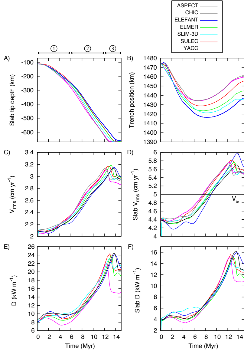
FIGURE 4.3 – Results of 7 codes for case 1 linear viscous models. A) Slab tip depth. B) trench position. Root-mean-square velocity (Eq. 4.12) for C) the whole model and D) the subducting slab only. Viscous rate of dissipation of energy (Eq. 4.14) for E) the whole mantle and F) the subducting slab only. In panels E) and F) the data is smoothed with a Bezier curve of degree n (the number of data points) that connects the endpoints. The smoothing is used to aid the visualization of the plot.
