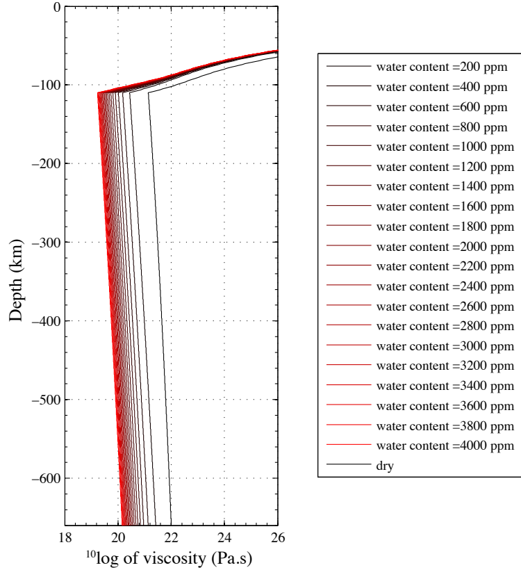
FIGURE 2.5 – Viscosity (Eq. 2.7) as a function of depth calculated using a constant strain rate of 10^{-15} \text{ s}^{-1} , a water content ranging from 0 to 4000 ppm, and the values in Hirth and Kohlstedt (2003) (Table 2.1).
