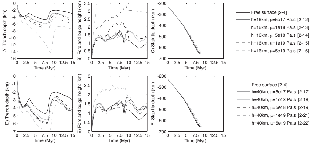
FIGURE 3.11 – Quantification of results from ocean-ocean type models including a 'sticky air' layer. A), D) Maximum trench depth, B), E) maximum foreland bulge height and C), F) slab tip depth as a function of time using symmetrical in- and outflow lateral boundary conditions. The surface boundary is either (1) free or (2) free-slip which includes a 'sticky air' layer with variable viscosities. The top three panels (A, B and C) are for models with a 16 km thick 'sticky air' layer and the bottom three panels (D, E and F) are for a 40 km thick 'sticky air' layer.
