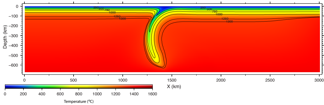
FIGURE 4.6 – Temperature distribution at t=12.5 Myr for linear viscous case 2 model, computed with SULEC.
