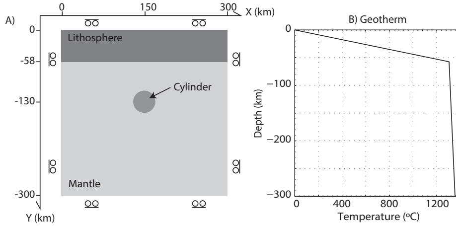
FIGURE 5.5 – (A) Model setup for a cold, hydrated cylinder sinking in a warm, dry mantle. All materials are linear viscous and their rheological parameters are given in Table 5.2. (B) Initial geotherm for model in (A).
