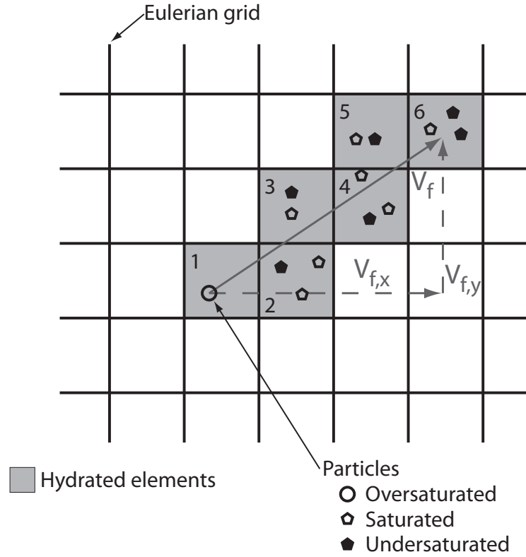
FIGURE 2.4 – Schematic migration of free water and its distribution along a prescribed path for our velocity controlled water migration schemes 2 and 3 (see text for further explanation). V_f is water velocity.
