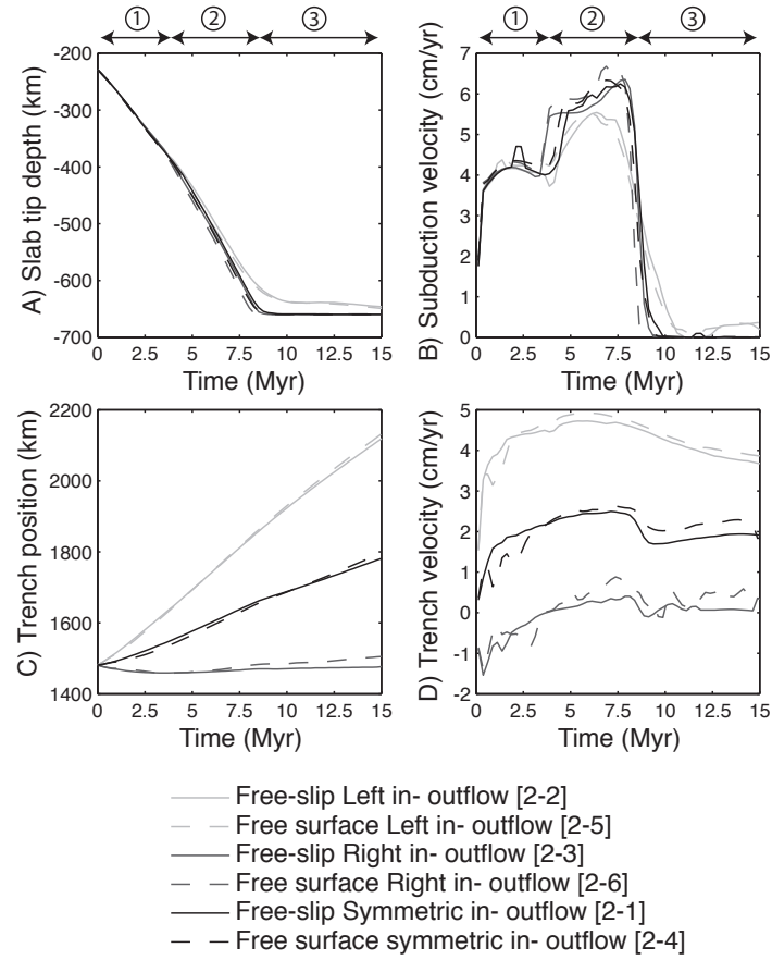
FIGURE 3.6 – Quantification of results for ocean-ocean models. A) Slab tip depth, B) vertical velocity of the slab tip, C) trench horizontal position and D) trench migration velocity as a function of time. The lateral boundary conditions are left material inflow, right material inflow, or left and right material inflow. The surface boundary condition is either free-slip or a free surface and the bottom boundary condition is free-slip. The circled numbers at the top of each column denote the subduction phases. A minor spline-type of smoothing is applied to the velocity curves to take out the small wavelength fluctuations caused by particle motions (panels B and D).
