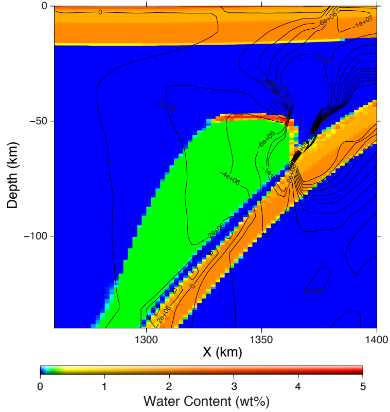
FIGURE 5.4 – A close up of the mantle wedge region at 5 Myr in a subduction model that uses free water migration scheme I in which viscosity decreases with bound water content. Shown is the elemental bound water content with contours at every 2 MPa of the horizontal pressure difference, \frac{dP}{dx} . Horizontal pressure variations are low in the region with highest bound water content.
