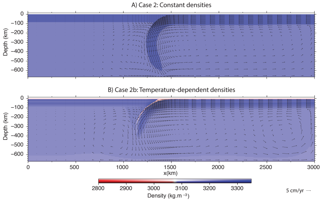
FIGURE 4.9 – Linear viscous model densities and nodal velocities at 12 Myr for A) case 2 linear viscous model with constant densities, and B) case 2b, linear viscous model with temperature-dependent densities. The models were calculated using SULEC.
