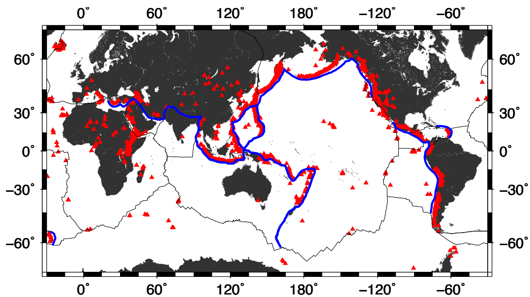
FIGURE 1.1 – Map of the plate boundaries (black lines) and subduction zones (blue lines), as defined in NUVEL-1A (DeMets et al., 1994). The location of volcanoes are in red (Siebert and Simkin, 2002). Most volcanoes are grouped into curved arcs (the volcanic arcs or island arcs) that are parallel to the trenches. This is particularly visible around the Pacific plate, the so-called ‘Ring of fire’.
