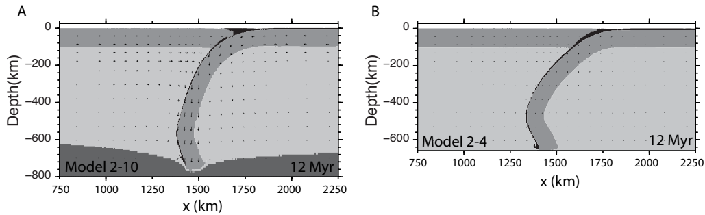
FIGURE 3.7 – The effect of adding a linear viscous lower mantle to ocean-ocean subduction models. The models have symmetric material in- and outflow. A) A 500 km thick lower mantle and B) without lower mantle.
