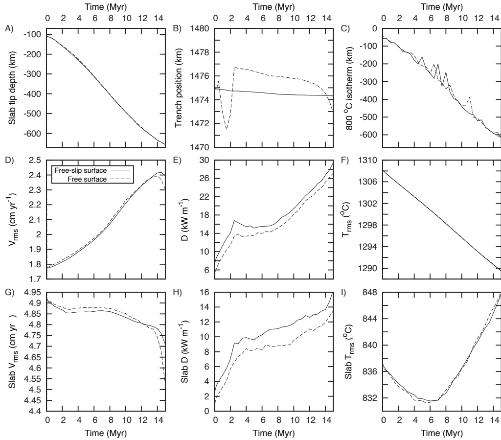
FIGURE 4.15 – Results for thermo-mechanical models (case 4) using SULEC with either a free-slip surface or a free surface. A) Slab tip depth. B) trench position. C) Depth of the 800 °C isotherm. Whole model D) root-mean-square velocity (Eq. 4.12), E) Viscous rate of dissipation of energy (Eq. 4.14), and F) root-mean-square temperature (Eq. 4.15). Slab G) Root-mean-square velocity, H) Viscous rate of dissipation of energy, and I) Root-mean-square temperature.
