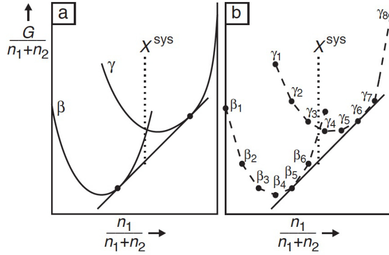
FIGURE 2.2 – Schematic isobaric-isothermal free energy-composition diagrams for a binary system illustrating the distinction between the non-linear solution to the phase equilibrium problem (a) and its linear approximation (b). Figure from Connolly (2005).
