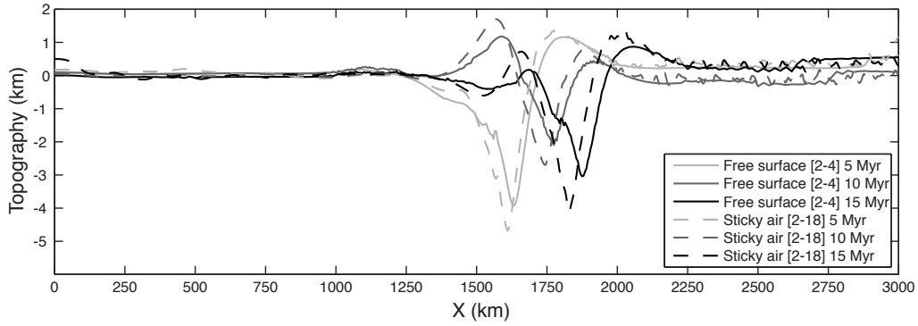
FIGURE 3.9 – A comparison of surface topography at 5, 10 and 15 Myr for a free surface model (model [2-4], solid lines) and a free-slip model with a 'sticky air' layer (model [2-18], dashed lines). The 'air' layer is 40 km thick and has a viscosity of 10^{18} Pa.s . The models have symmetric in- and outflow and only differ in the absence/presence of the 'sticky air' layer.
