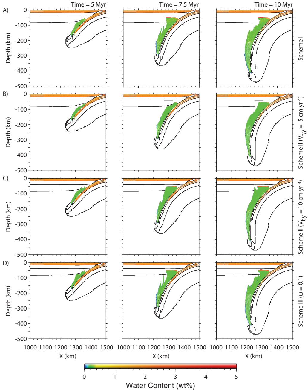
FIGURE 5.10 – Bound water distribution for subduction models after 5, 7.5 and 10 Myr for the following free water migration schemes: (A) Elemental water migration scheme I (velocity v_{f,y} increases from 10 \text{ cm yr}^{-1} just below the lithosphere to 70 \text{ cm yr}^{-1} at the base of the model where the grid is coarsest); (B) imposed vertical velocity v_{f,y} = 5 \text{ cm yr}^{-1} (scheme II); (C) imposed vertical velocity v_{f,y} = 10 \text{ cm yr}^{-1} and (D) Darcy velocity with efficiency factor \omega = 0.1 (scheme III). Bound water moves with the solid phase flow. Viscosity of all materials changes with water content following the flow law of Eq. 5.4.
