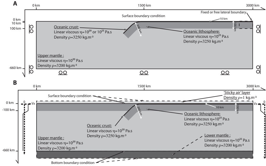
FIGURE 3.1 – A) Gravitational subduction model setup. Lateral and bottom boundary conditions are free-slip. The surface boundary condition is either free surface or free-slip. The subducting lithosphere is either held fixed at its lateral edge or it can be decoupled (dashed box is filled with mantle material in the latter case). B) Ocean-ocean type model setup. The bottom boundary condition is free-slip and can include a linear viscous lower mantle of variable thickness. The lateral boundary conditions include material in- and outflow. The surface boundary condition is either (1) free surface, (2) free-slip or (3) reproducing a free surface using a free-slip model surface and a 'sticky air' layer.
