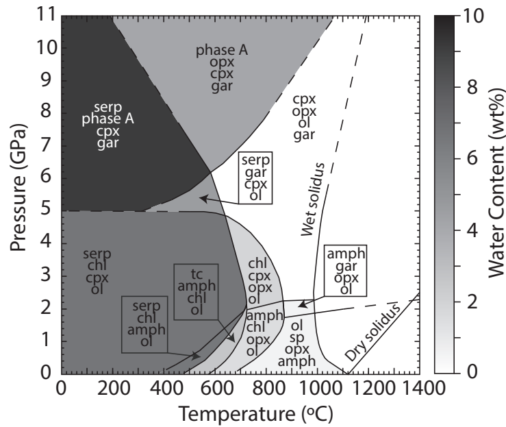
FIGURE 5.2 – Water content as a function of pressure and temperature for mantle material of pyrolitic composition, modified from Schmidt and Poli (1998). The solid lines are experimentally determined Clapeyron slopes (Schmidt and Poli, 1998), while the dashed lines have been extrapolated in a similar manner to Arcay et al. (2005). amph: amphibole; chl: chlorite; cpx: clinopyroxene; gar: garnet; opx: orthopyroxene; ol: olivine; serp: serpentine; sp: spinel; tc: talc.
