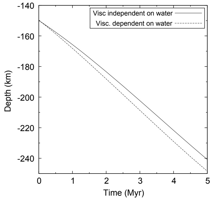
FIGURE 5.8 – Depth of the bottom of the subducting cylinder versus time for linear viscous models with or without including the effects of water on viscosity. This figure is for models that follow free water migration scheme I (Fig. 5.7a-c).
