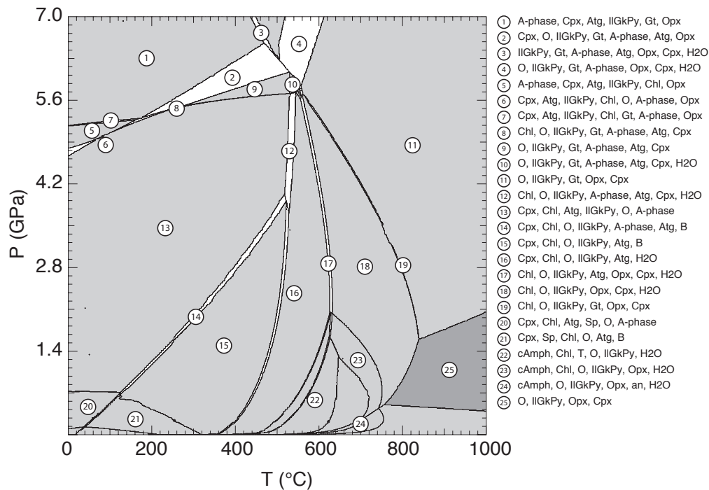
FIGURE 1.7 – Phase diagram for a Serpentinized Hartzburgite calculated using Perple_X (Connolly, 2005) by Zurab Chemia (Chemia et al., 2010). The phases are: A-phase, Cpx = Clinopyroxene, Atg = Antigorite, IlGkPy = Ilmenite, Gt = Garnet, Opx = Orthopyroxene, H 2 O = Water, O = Olivine, Chl = Chlorite, B = Brucite, cAmph = Clinoamphibole, Sp = Spinel, T = Talk, an = Anorthite.
