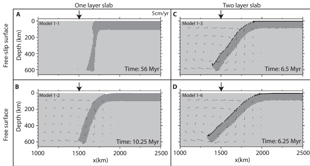
FIGURE 3.2 – A snapshot of four gravitational subduction models, with the slab held fixed at its right hand side, taken when the slab tip reaches a depth of 600 km. The central part of the total model width of 3000 km is shown. The black arrows at the surface of the model domain represent the initial position of the trench. A) A one layer lithosphere with a free-slip surface; B) a one layer lithosphere with a free surface; C) a two layer lithosphere with a free-slip surface and D) a two layer lithosphere with a free surface. The two layer models (C and D) differ from the one layer models (A and B) by inclusion of a weak crust. The time required to reach a depth of 600 km is indicated at the lower right of each frame. The one-layer lithosphere with a free-slip surface (A) subducts substantially slower than the other models. The model setup is shown in figure 3.1A.
