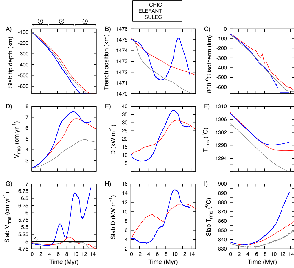
FIGURE 4.11 – Results for simplified case 3 thermo-mechanical models. A) Slab tip depth. B) trench position. C) Depth of the 800 °C isotherm. Whole model D) root-mean-square velocity (Eq. 4.12), E) Viscous rate of dissipation of energy (Eq. 4.14), and F) root-mean-square temperature (Eq. 4.15). Slab G) Root-mean-square velocity, H) Viscous rate of dissipation of energy, and I) Root-mean-square temperature.
