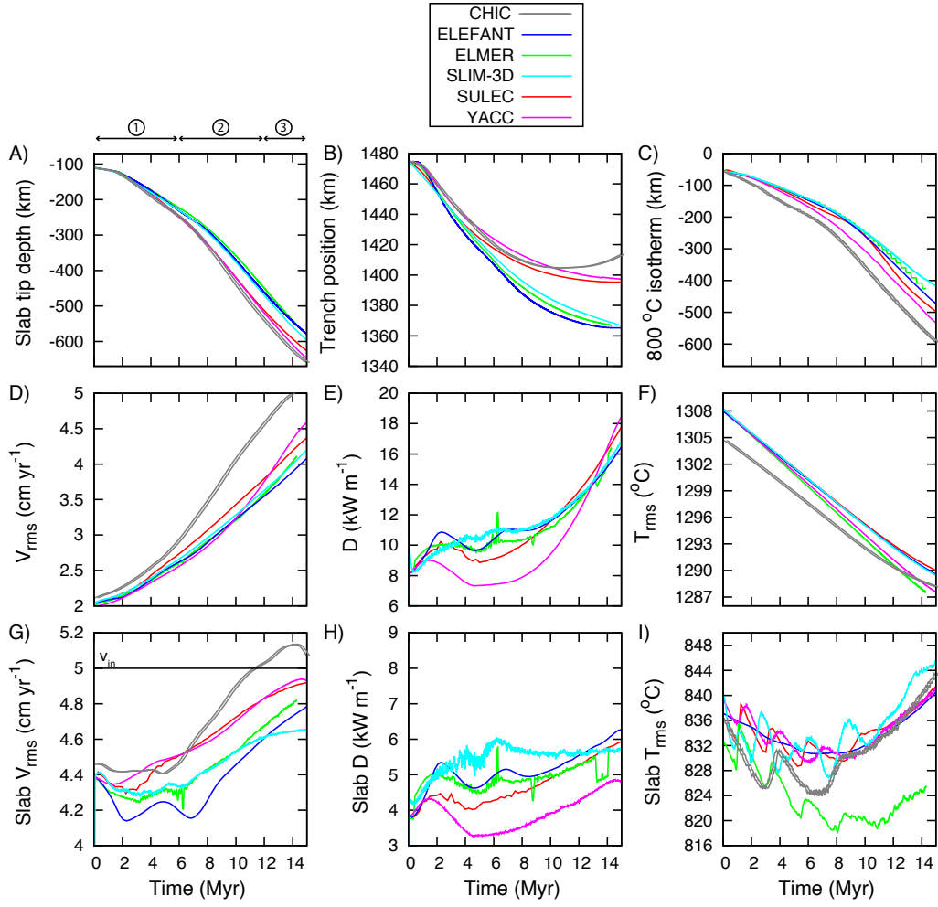
FIGURE 4.8 – Results for case 2b, linear viscous models with temperature-dependent densities. A) Slab tip depth. B) Trench position, C) Depth of the 800 °C isotherm. Whole model D) root-mean-square velocity (Eq. 4.12), E) Viscous rate of dissipation of energy (Eq. 4.14), and F) root-mean-square temperature (Eq. 4.15). Slab G) Root-mean-square velocity, H) Viscous rate of dissipation of energy, and I) Root-mean-square temperature.
