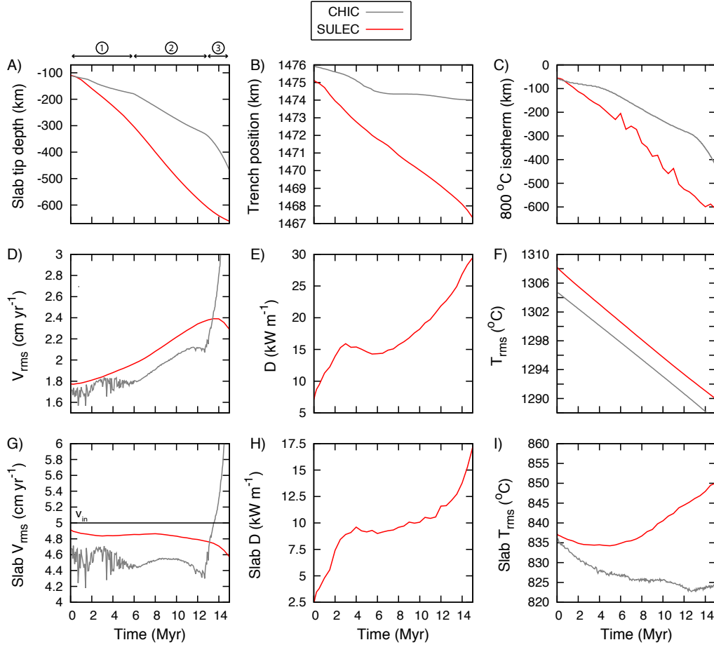
FIGURE 4.12 – Results for case 4 thermo-mechanical models. A) Slab tip depth. B) trench position. C) Depth of the 800 °C isotherm. Whole model D) root-mean-square velocity (Eq. 4.12), E) Viscous rate of dissipation of energy (Eq. 4.14), and F) root-mean-square temperature (Eq. 4.15). Slab G) Root-mean-square velocity, H) Viscous rate of dissipation of energy, and I) Root-mean-square temperature.
