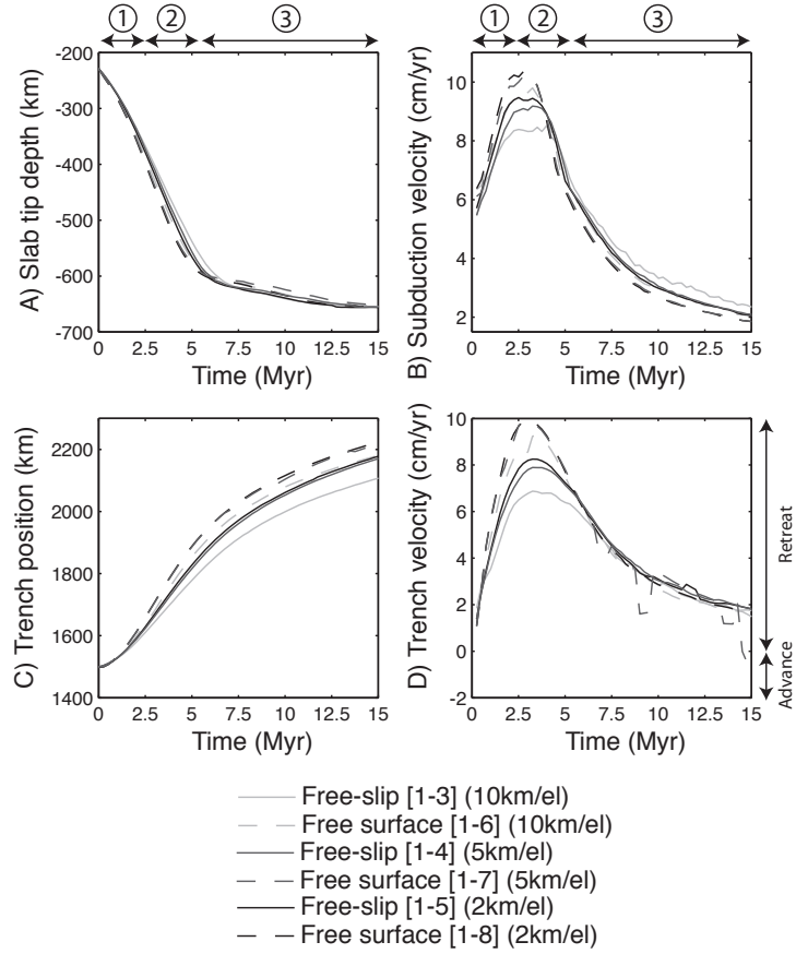
FIGURE 3.3 – Quantification of results for the gravitational subduction models. A) Slab tip depth, B) vertical velocity of the slab tip, C) trench horizontal position and D) trench migration velocity as a function of time using different mesh resolutions at the trench and different surface boundary conditions. The circled numbers at the top of each column denote the subduction phases. A minor spline-type of smoothing is applied to the velocity curves to take out the small wavelength fluctuations caused by particle motions (panels B and D).
