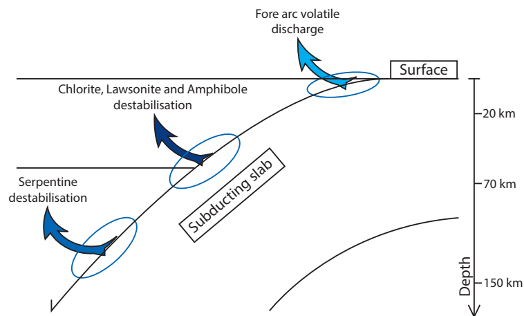
FIGURE 1.6 – Cartoon of the main dehydration processes occurring during subduction.
