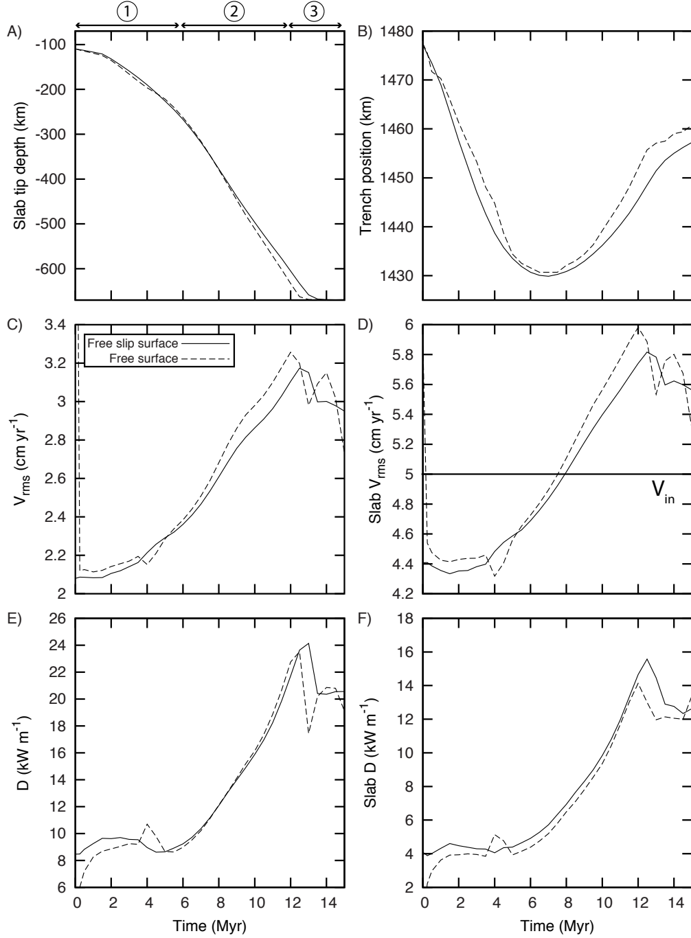
FIGURE 4.14 – Results for linear viscous case 1 models using SULEC with either a free-slip surface or a free surface. A) Slab tip depth. B) trench position. Root-mean-square velocity (Eq. 4.12) for C) the whole model and D) the subducting slab only. Viscous rate of dissipation of energy (Eq. 4.14) for E) the whole mantle and F) the subducting slab only.
