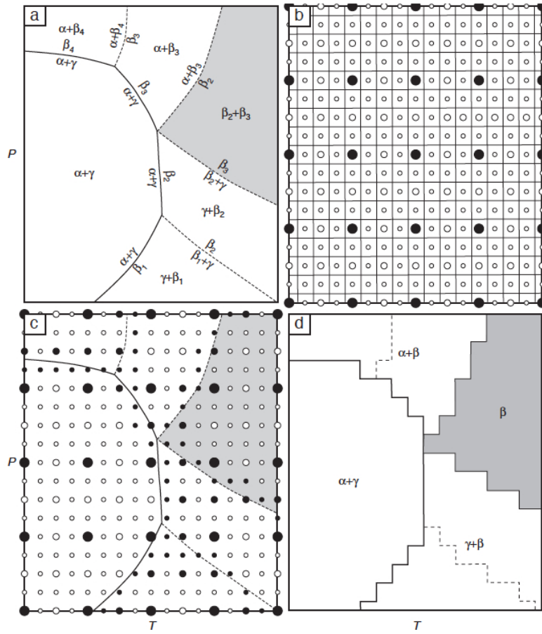
FIGURE 2.3 – Mapping algorithm used in Perple_X illustrated with schematic phase pressure-temperature diagram for a binary system; (a) the solution phase \beta is represented by pseudocompounds where the boundaries between pseudocompounds (the dotted lines) can approximate true phase boundaries or a difference in composition (the boundaries of the dark gray area) or homogeneous equilibration of a solution as a function of pressure and temperature; (b) Phase relations are mapped by sampling on a four level grid, with grid nodes at progressively higher levels indicated by circles of decreasing size; (c) The nodes at which phase relations would be computed as dictated by the mapping strategy are indicated by filled circles. The algorithm assigns the assemblages associated with the open circles; (d) the final map of the section is constructed by assuming that each node of the grid represents a finite area of the diagram. Figure from Connolly (2005) .
