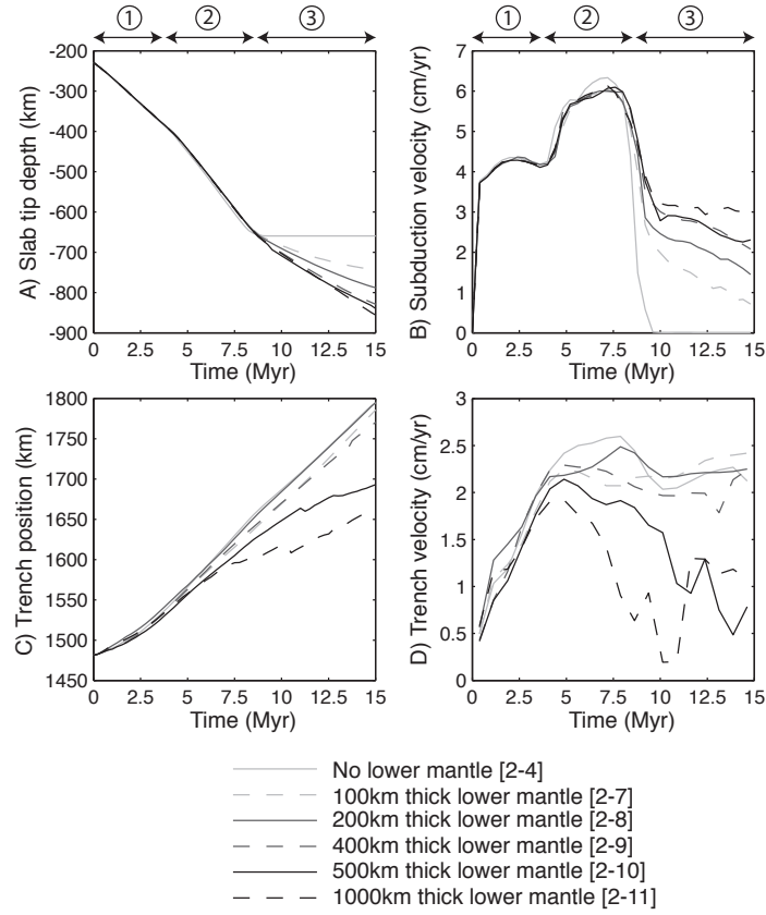
FIGURE 3.8 – Quantification of the effect of adding a lower mantle on A) Slab tip depth, B) vertical velocity of the slab tip, C) trench horizontal position and D) trench migration velocity as a function of time for symmetric ocean-ocean subduction models with a free surface. The bottom boundary condition is free-slip. The thickness of the linear viscous lower mantle is varied between 0 (no lower mantle) and 1000 km. The circled numbers at the top of each column denote the subduction phases. A minor spline-type of smoothing is applied to the velocity curves to take out the small wavelength fluctuations caused by particle motions (panels B and D).
