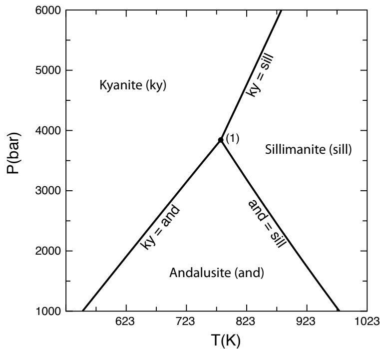
FIGURE 2.1 – A simple example of a one component phase diagram calculated for aluminosilicates ( \text{Al}_2\text{SiO}_5 ) using Perple_X . Three solid phases are present, that are polymorphs of \text{Al}_2\text{SiO}_5 : andalusite, kyanite and sillimanite. Point (1) is the invariant point where the three univariant curves ( i.e. , the reaction curves, \text{ky} = \text{and} , \text{and} = \text{sill} , \text{ky} = \text{sill} ) intersect.
