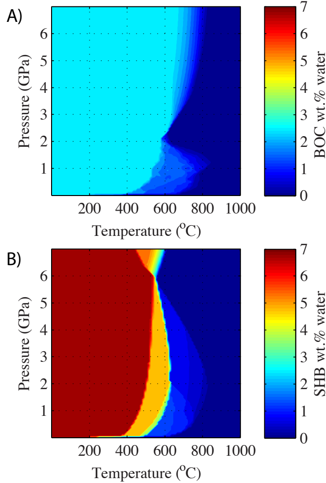
FIGURE 5.1 – Water content as a function of pressure and temperature calculated using Perple_X for (A) Bulk Oceanic Crust, and (B) Serpentinised Harzburgite lithologies ( Chemia et al., 2010 ). Bulk compositions are in Table 5.1.
