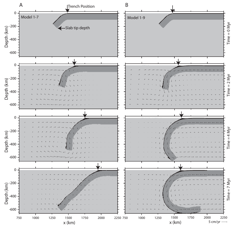
FIGURE 3.4 – Snapshots of the evolution through time of a two-layer gravitational subduction model with a free surface. The models include a subducting lithosphere that is A) 'coupled' or B) 'decoupled' to the right hand side boundary. The elemental material distribution and a sample of the nodal velocities are shown (the velocity scale is at the lower right). See text for further description.
