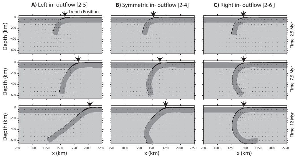
FIGURE 3.5 – Snapshots at 2.5, 7.5 and 12 Myr for ocean-ocean convergence models. The top boundary is a free surface, the bottom boundary is free-slip and the lateral boundaries are varied between A) in- and outflow from the left hand side, B) symmetric in- and outflow and C) in- and outflow from the right hand side. The model numbers are given in brackets.
