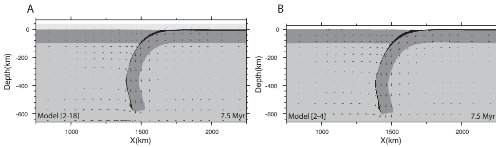
FIGURE 3.10 – Snapshot of ocean-ocean type subduction models at 7.5 Myr with A) a 'sticky air' layer (40 km thick and 10^{18} Pa.s viscosity) or B) a free surface, showing that 'sticky air' models reproduce the overall characteristics of models with a free surface. The model has symmetric in- outflow lateral boundary conditions.
