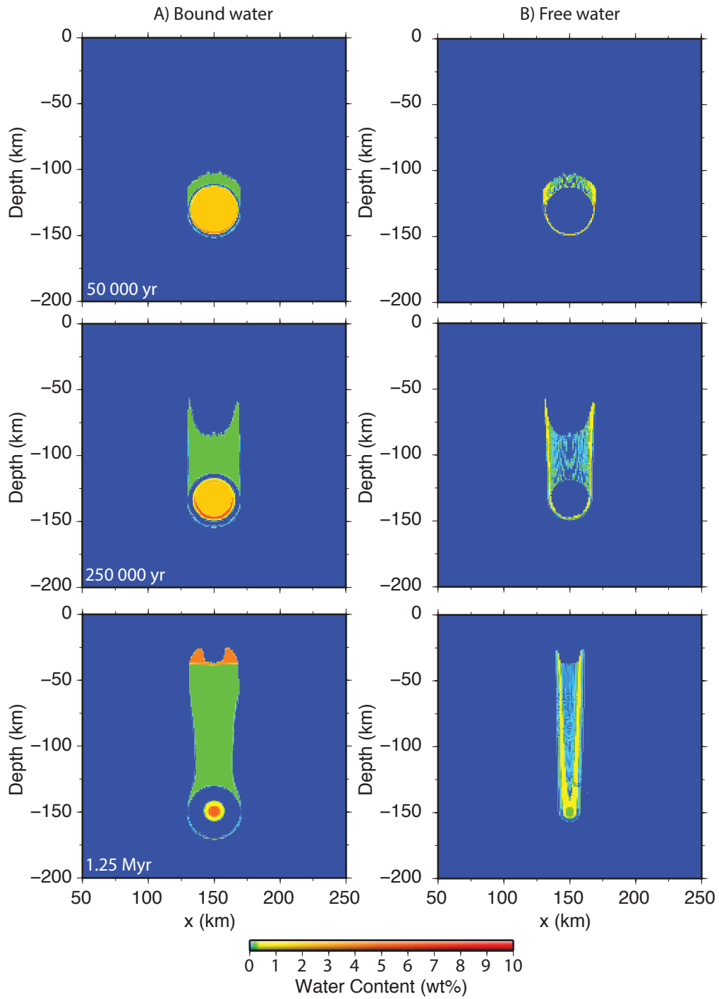
FIGURE 5.6 – Elemental water content for the Stokes flow models using scheme I (20 cm yr -1 ) for a grid resolution of 1 km × 1 km showing (A) bound water, and (B) free water.
