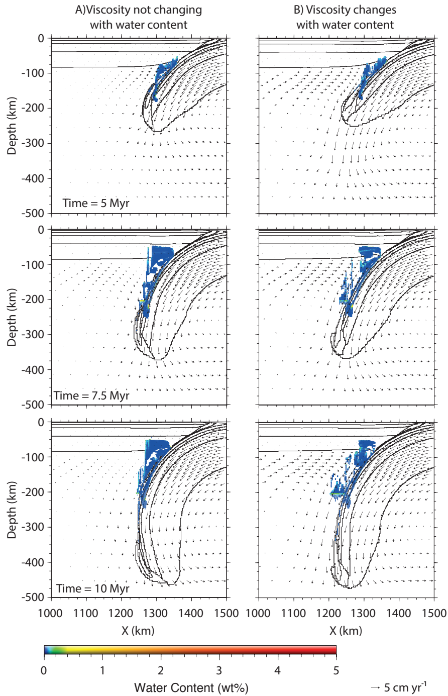
FIGURE 5.14 – Bound water distribution for subduction models using Darcy free water migration scheme III (with efficiency factor \omega = 0.1 ) at 5, 7.5 and 10 Myr. (A) Water content does not change viscosity; (B) water content decreases the viscosity (following flow law Eq. 5.4).
