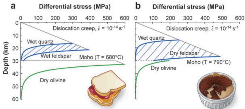
FIGURE 1.5 – The two strength profiles of the lithosphere: a) Jelly sandwich characterised by a weak lower crust and a strong uppermost mantle or b) Crème brûlée where the uppermost mantle is weak (which could result from a high geotherm, 90 \text{ mW m}^{-2} , or the addition of water). Figure from Bürmann and Dresen (2008).
