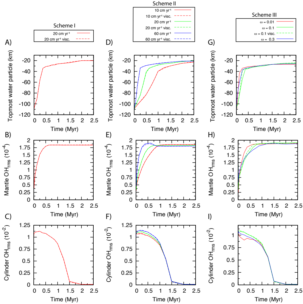
FIGURE 5.7 – Evolution with time of the depth of the top-most particle of hydrated material (top row), mantle \text{OH}_{\text{rms}} (middle row) and cylinder \text{OH}_{\text{rms}} (bottom row) for our models of a wet sinking cylinder. The first column show results for scheme I (water migration velocity of 20 \text{ cm yr}^{-1} ), the second for scheme II with different imposed velocities ( v_{f,y} = 10, 20 and 60 \text{ cm yr}^{-1} ) and the third for scheme III in which the water migration velocity is calculated using the Darcy law with efficiency factor \omega = 0.01, 0.1 or 0.3 (Sect. 2.3). Models labelled “visc” have a decrease in viscosity with increasing water content.
