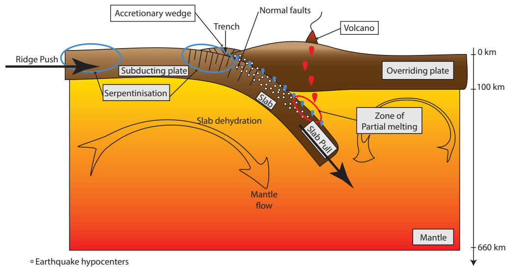
FIGURE 1.2 – Cartoon of the main processes occurring in a subduction system.
