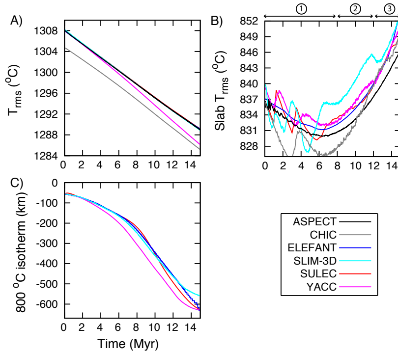
FIGURE 4.7 – Results for case 2, linear viscous models with temperature advection but with constant densities. A) root-mean-square temperature (Eq. 4.15). B) Slab root-mean-square temperature. C) Depth of the 800 °C isotherm.
