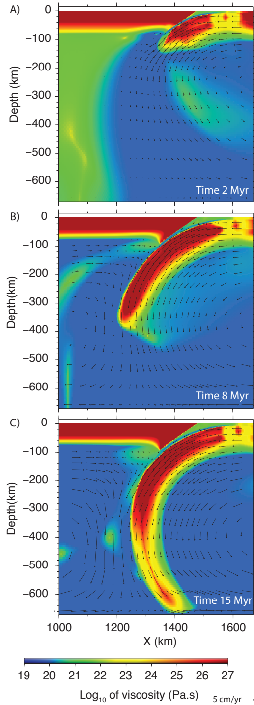
FIGURE 4.10 – Viscosity fields at A) 2, B) 8 and C) 15 Myr for thermo-mechanical case 3. The model was calculated using SULEC.
