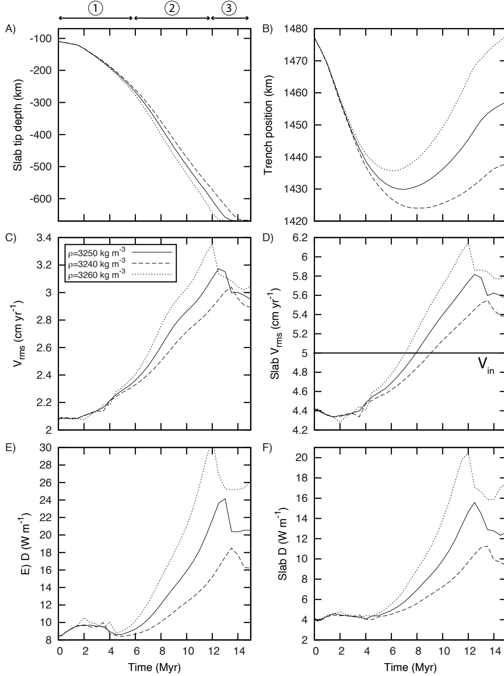
FIGURE 4.16 – Results for linear viscous models with different lithospheric densities. The mantle density is fixed at 3200 \text{ kg m}^{-3} . Models are calculated using SULEC. A) Slab tip depth. B) Trench position. Root-mean-square velocity (Eq. 4.12) for C) the whole model and D) the subducting slab only. Viscous rate of dissipation of energy (Eq. 4.14) for E) the whole mantle and F) the subducting slab only. The models in this study use \rho=3250 \text{ kg m}^{-2} .
