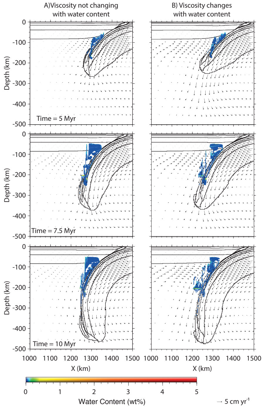
FIGURE 5.15 – Free water distribution for subduction models using the Darcy water migration scheme (with \omega = 0.1 ) at 5, 7.5 and 10 Myr. (A) Water content does not change viscosity; (B) water content decreases the viscosity (following flow law Eq. 5.4).
