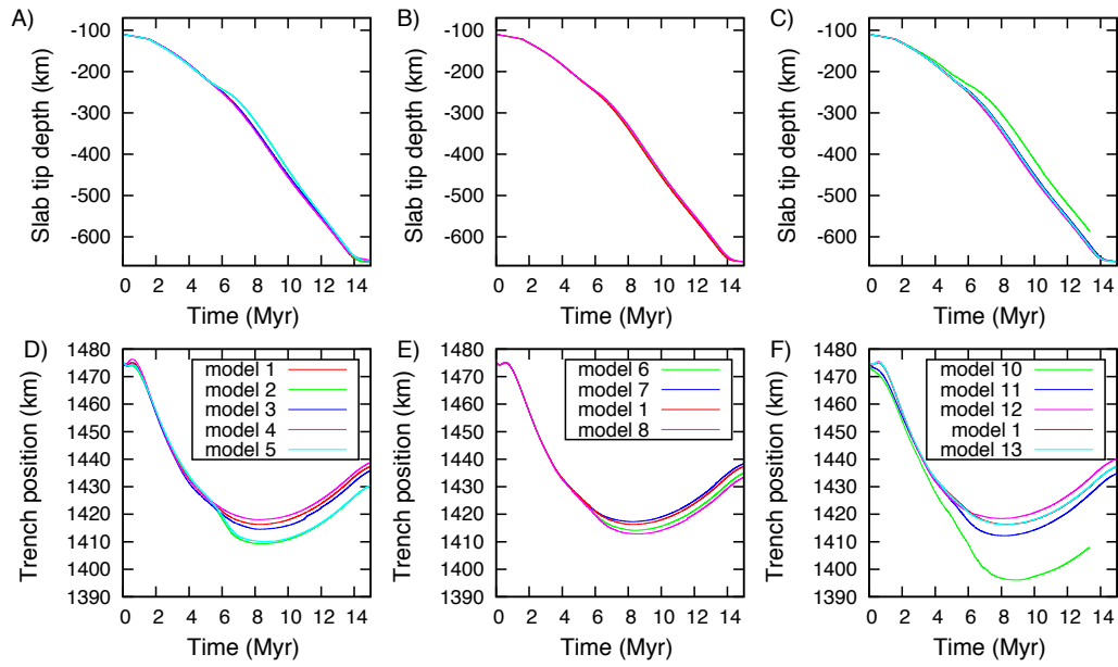
FIGURE 4.5 – Slab tip depth and trench position for a series of case 1 linear viscous models that investigate the effects of grid resolution (the number of elements), particle density and penalty parameter ( B in Eq. 4.10) computed with ELEFANT. The models are described in table 4.4
