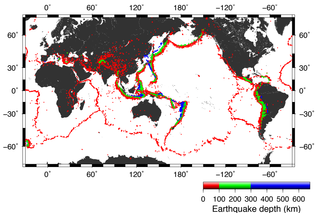
FIGURE 1.3 – Location of upper mantle earthquakes (down to a depth of 670 km) with a magnitude over 4.5 that occurred over the last 5 years. Shallow earthquakes are in red, intermediate earthquakes in green, and deep earthquakes in blue. The earthquake database is from NEIC http://earthquake.usgs.gov/earthquakes/ . The polarity of subduction is shown by the distribution of earthquakes, the deep earthquakes are located furthest away from the trench.
