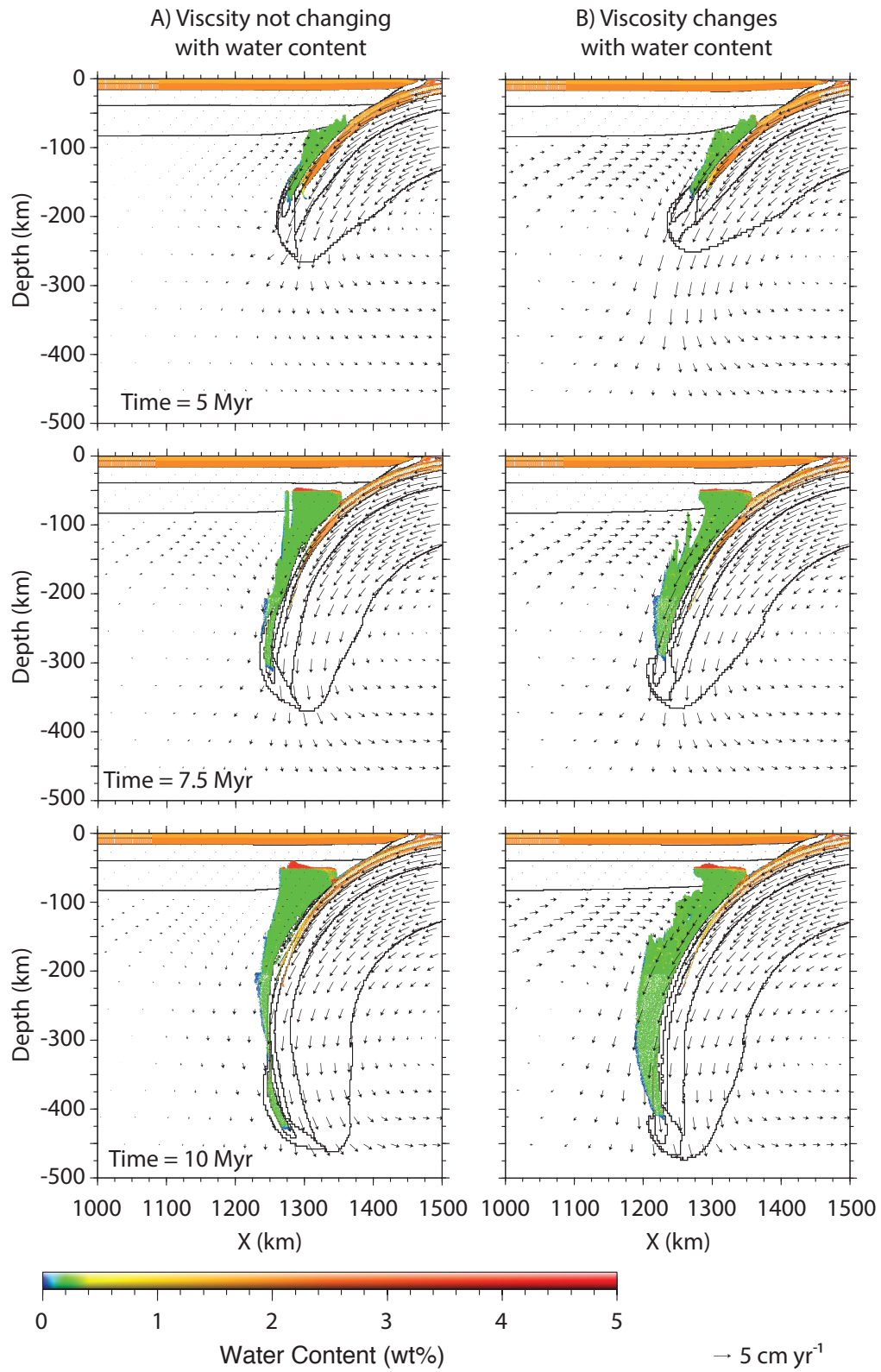
FIGURE 5.13 – Viscosity field for models that follow the Darcy free water migration scheme III with efficiency factor \omega = 0.1 after 7.5 Myr for: (A) viscosity not dependent on water content, and (B) viscosity decrease with water content.
