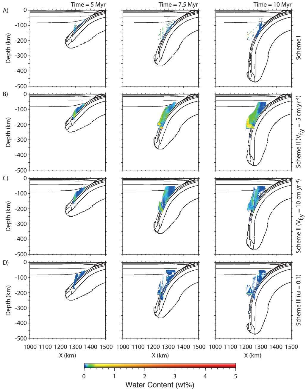
FIGURE 5.11 – Free water distribution for subduction models after 5, 7.5 and 10 Myr for the following water migration schemes: (A) Elemental water migration scheme I (velocity v_{f,y} varies between 10 and 70 \text{cm yr}^{-1} ); (B) Imposed vertical water migration scheme II with v_{f,y} = 5 \text{ cm yr}^{-1} ; (C) Imposed vertical water migration scheme II with v_{f,y} = 10 \text{ cm yr}^{-1} , and (D) Darcy water migration scheme III with efficiency factor \omega = 0.1 . Viscosity of all materials changes with water content following flow law of Eq. 5.4.
