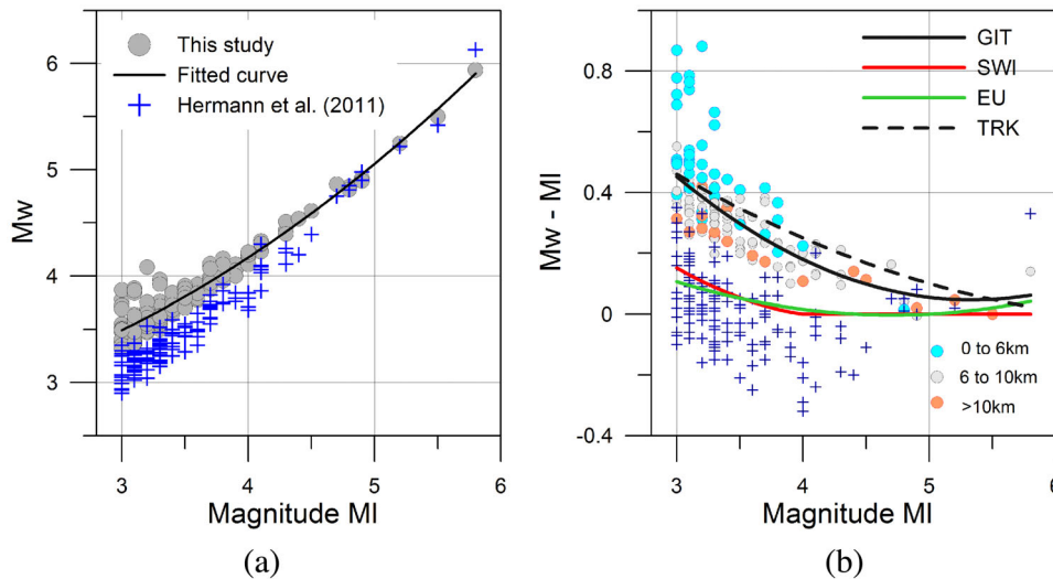
Figure 10. (a) Moment magnitude ( M_w ) estimated from the inverted source spectra (circles) versus local magnitude ( M_I ). The black line represents the quadratic model. The blue crosses indicate the M_w values estimated by Herrmann et al. (2011). (b) Magnitude difference M_w - M_I versus M_I . The circles are the difference computed considering the M_w from this study, where the colours represent different depth intervals. The blue crosses are the difference computed considering the Herrmann magnitudes. The lines are different relationships between M_w and M_I . Continuous black: the best fit for this study; dashed black: Parolai et al. (2007) model shifted by 0.5 magnitude units; green and red lines: Grünthal et al. (2009) and Goertz-Allmann et al. (2011) relationships, respectively, shifted by 0.3 M_w units.
