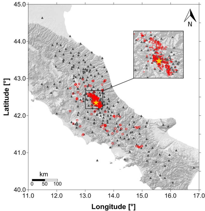
Figure 1. Locations of seismic events (red circles) and recording stations (triangles) considered in this study; the inset highlights the 2009 L'Aquila seismic sequence. The star is the epicentre of the M_w 6.1 main shock.
