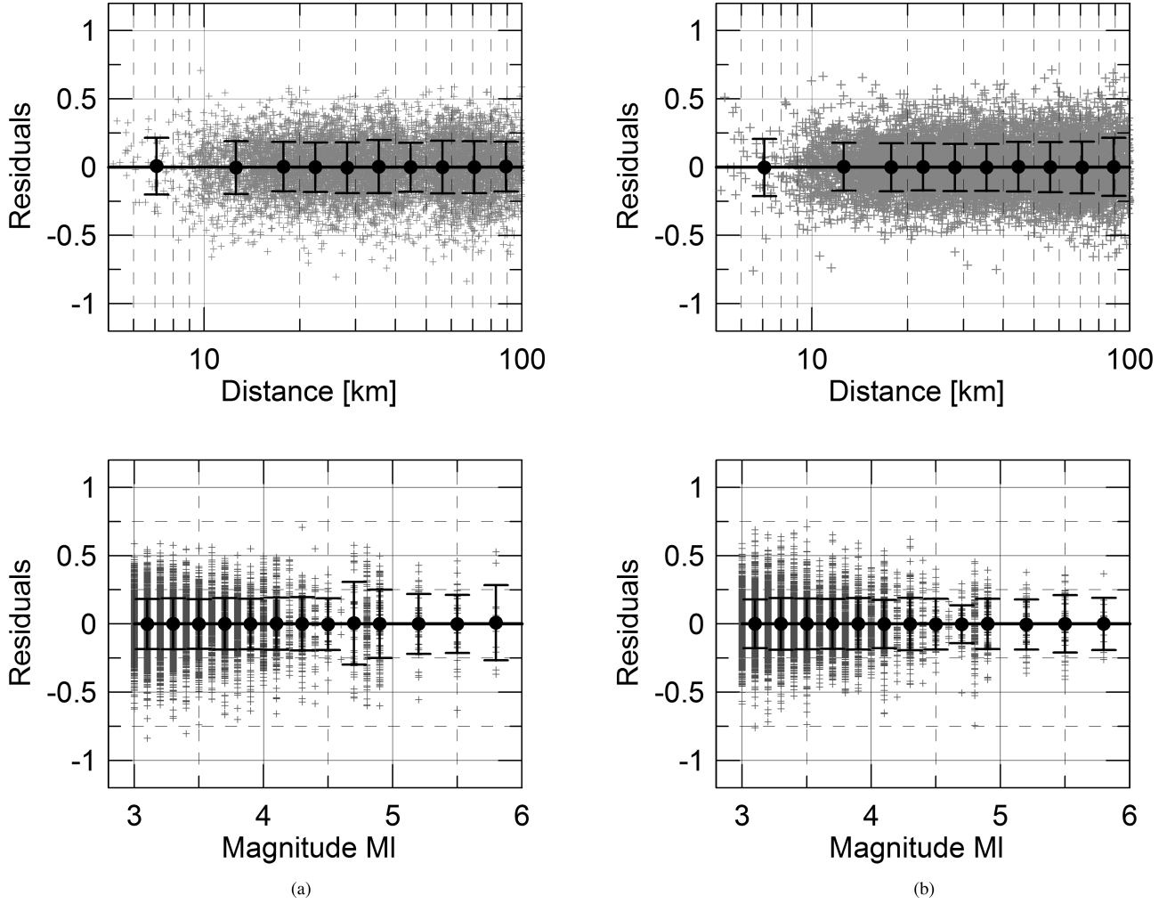
Figure 7. Residuals (grey symbols), computed as \log_{10}(\text{observation/prediction}) , at 1 Hz (a) and 10 Hz (b) as a function of distance (top) and magnitude (bottom); the mean residuals \pm one standard deviation computed for different distance and magnitude bins are shown as black dots with error bars.
