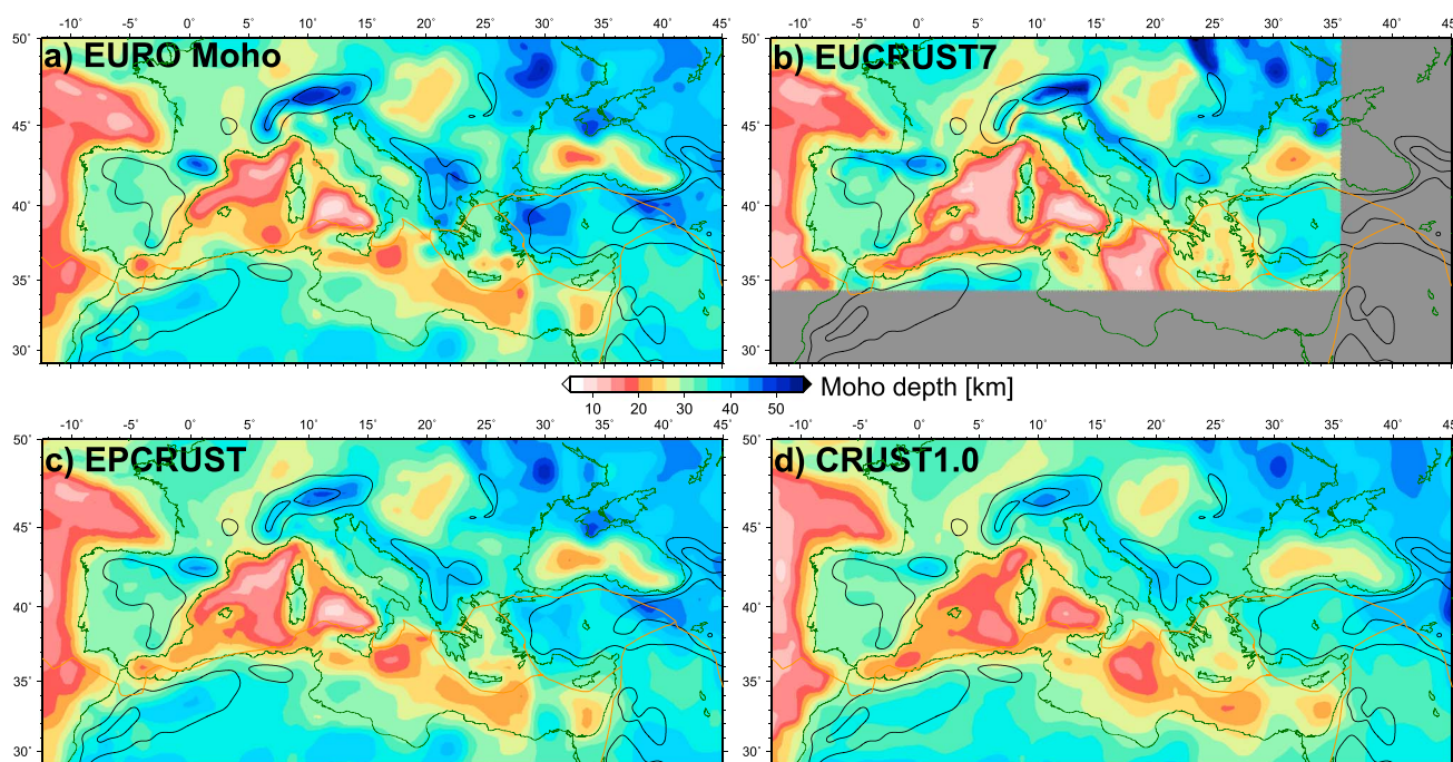
Figure 5. Comparison of crustal models for Moho depth. (a) EuroMoho [Grad et al. , 2009], (b) EuCrust07 [Tesauro et al. , 2008], (c) EpCrust [Molinari and Morelli, 2011], and (d) CRUST1.0 [Bassin et al. , 2000; Laske et al. , 2013]. Contours show long-wavelength (300 km Gaussian filter) smoothed, positive topography in 750 m contours to allow visual association of regions where high topography is mirrored by isostatically thickened crust.
